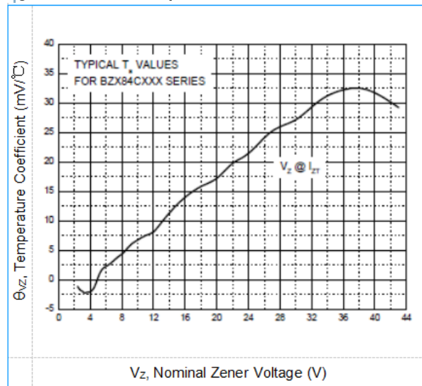
Fig3. Zener Diode Temperature Coefficients
