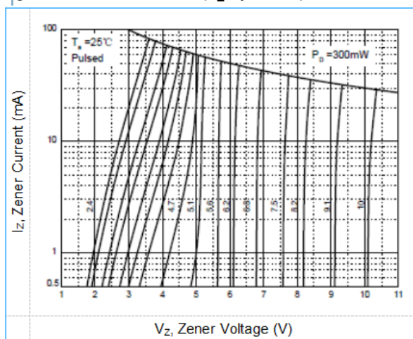
SOT-23 Surface Mount Zener Diode BZX84C27 Curves: Fig1. Zener Characteristics (V Z Up to 10V)
