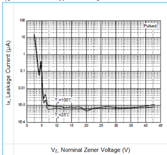
Fig4. Zener Diode Typical Leakage Current
