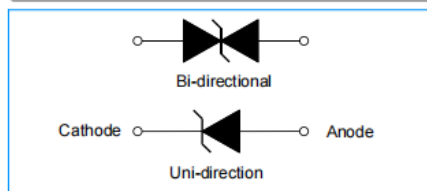
Functional Diagram
